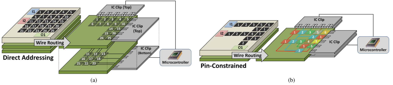
Fig. 5. DMFB typically has one or more PCB layers (green) beneath the electrode array which connect the microcontroller to the control electrodes. (a) Direct addressing DMFB is believed to require many PCB layers, while (b) pin-constrained DMFBs are designed to reduce the number of PCB layers.
