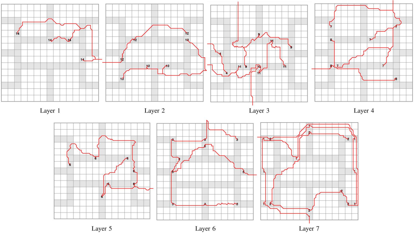
Fig. 17. Naïve method [38] routes the Zhao_PCR benchmark using seven PCB layers.
