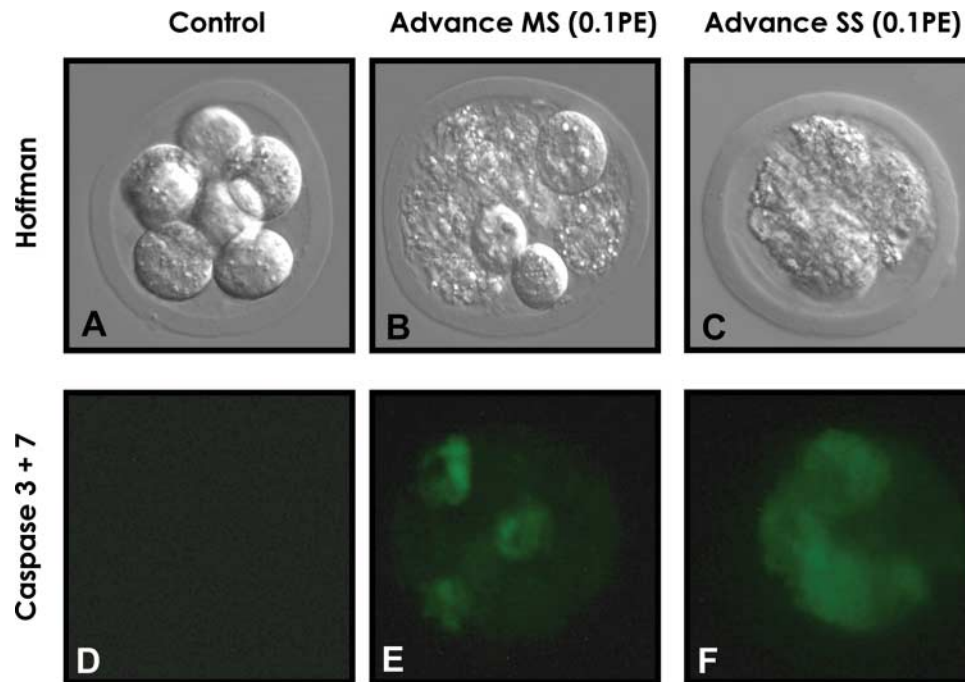
Figure 9 Smoke treatment induced apoptosis in mouse preimplantation embryos through activation of caspases 3 and 7. (A–C) Hoffman contrast images of preimplantation embryos incubated in control medium (A), 0.1 puff equivalents (PE) of Advance MS smoke solution (B), or 0.1PE of Advance SS smoke solution (C). (D–F) The same preimplantation embryos viewed with fluorescence microscopy to visualize activated caspases 3 and 7. (D) Absence of activated caspases 3 and 7 in blastomeres of control untreated embryo, (E) Presence of activated caspases 3 and 7 in embryo treated with Advance filtered MS smoke, (F) Detection of activated caspases 3 and 7 in embryo treated with SS smoke.
