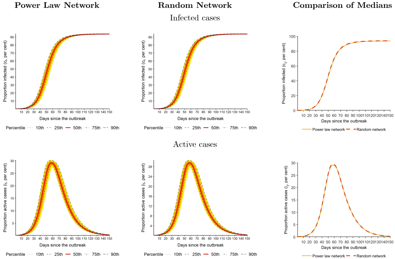
Figure S.3: Simulated number of infected and active cases using a single group model with \mathcal{R}_0 = 3 under different network topologies
