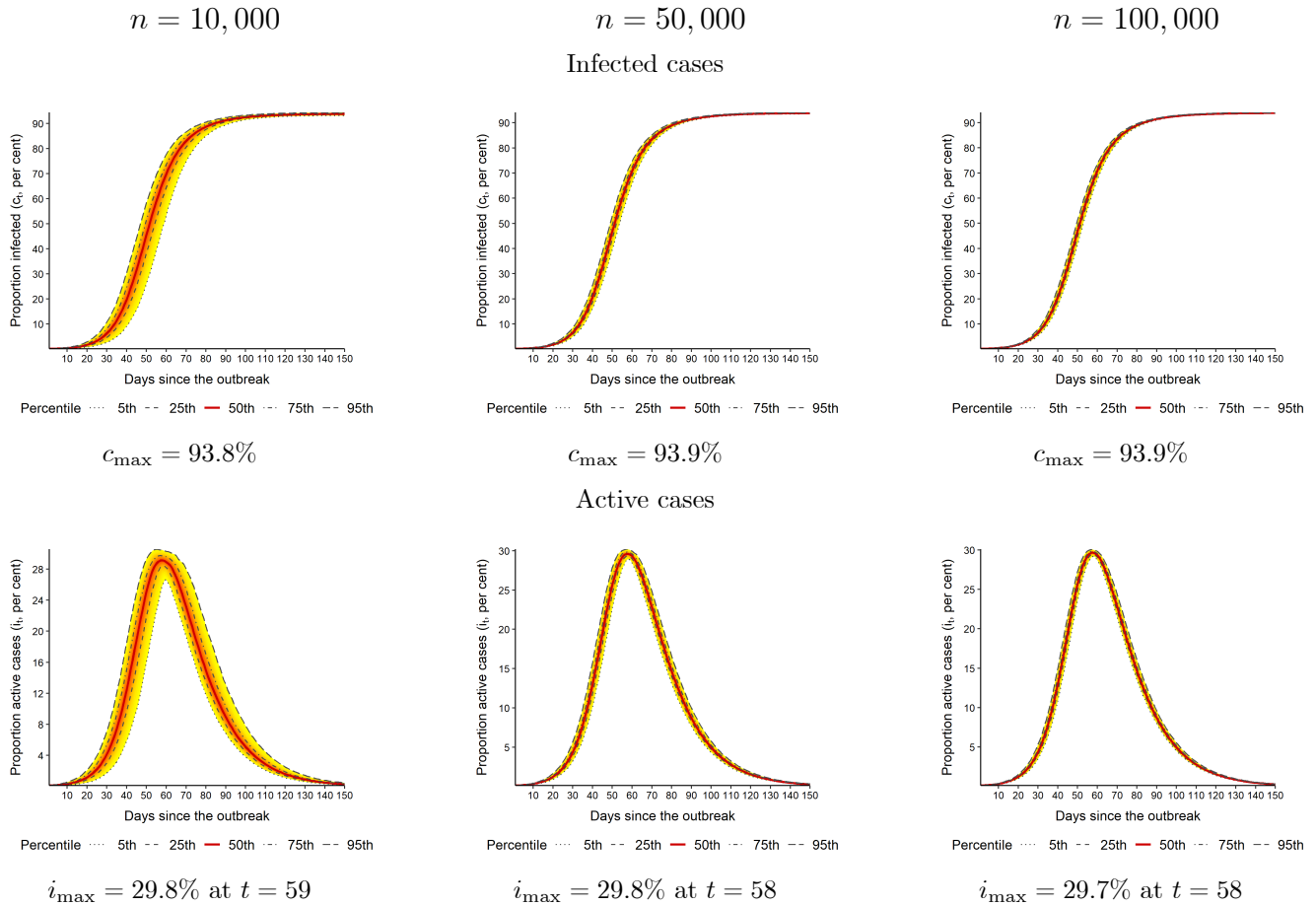
Figure S.1: Simulated number of infected and active cases using a single group model with \mathcal{R}_0 = 3 under different population sizes
