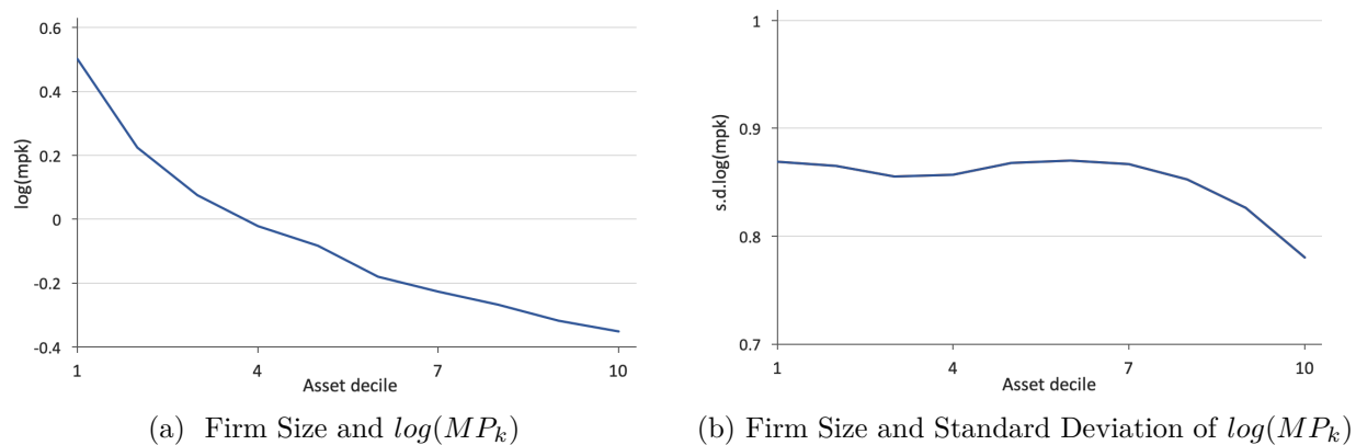
Figure 2: Firm Size and \log(MP_k)
