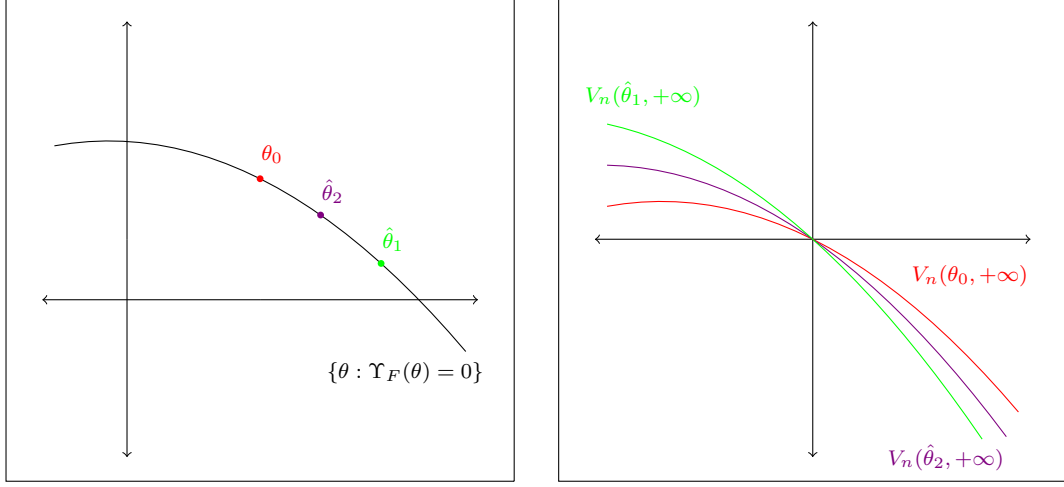
Figure 3: Approximating Impact of Equality Constraints
