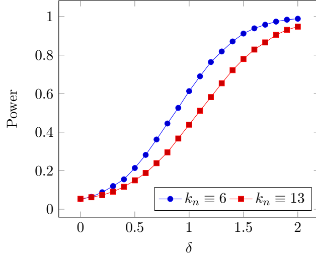
Figure 4: Monotonicity Test - Empirical Power
